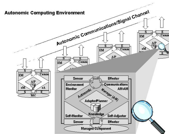
Figure 2 Autonomic System Environment consisting of Autonomic Elements
